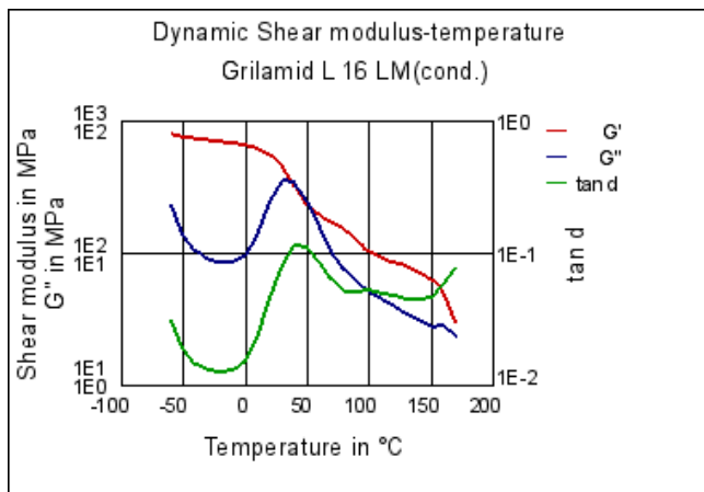
Dynamic Shear modulus-temperature
