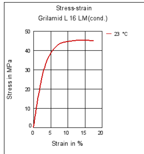
Stress-strain
